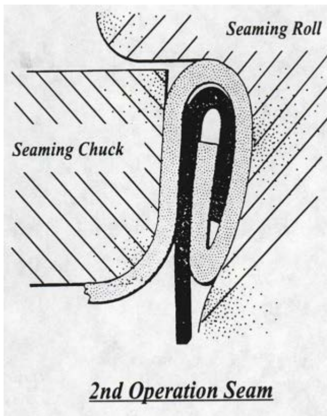
IMAGE 2 – 2 nd Operation
